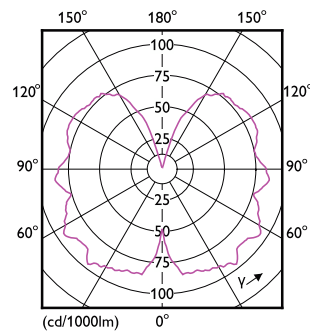
Light Distribution Diagram - 6.5ST19/VIN/820/E26/Amber/G/SP/D 1PFT20
