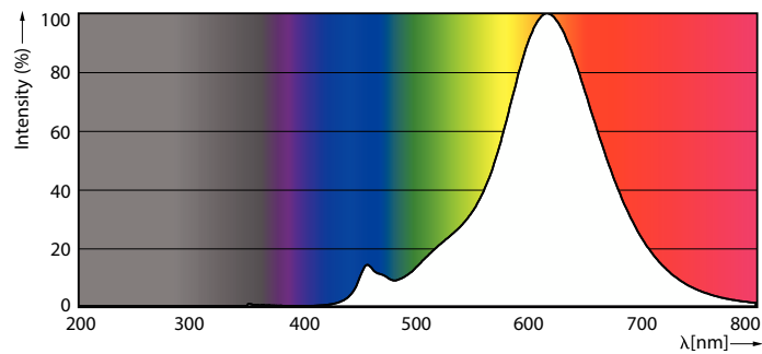
Spectral Power Distribution Colour - 6.5ST19/VIN/820/E26/Amber/G/SP/D 1PFT20
