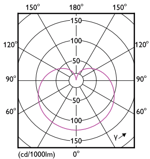
LEDBulb A19 E26 8.8-60W
