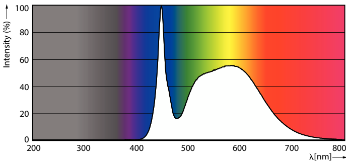
Spectral Power Distribution Colour - 80CC/LED/3CCT/LS EX39 BB 3/1
