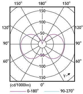
Light Distribution Diagram - 80CC/LED/3CCT/LS EX39 BB 3/1
