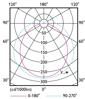
Light Distribution Diagram - 8PL-L/COR/18-5CCT/MF9/G/4P 10/1
