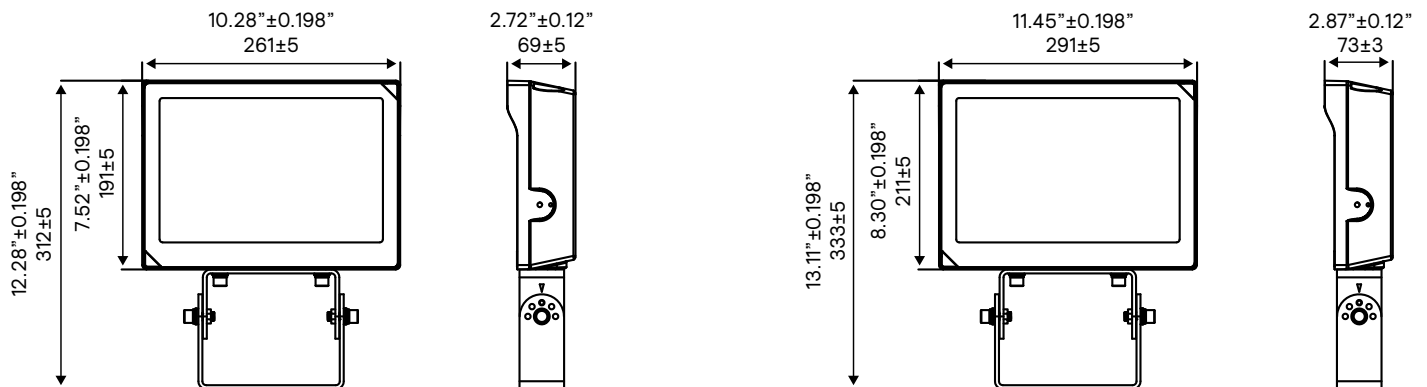
100W Trunnion Slim Flood 60–80–100W/3CCT/UN3/TN/PCB
