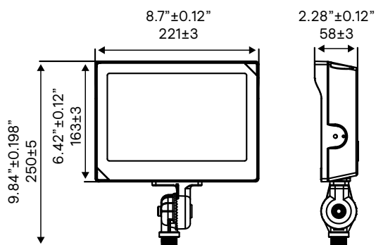
60W Knuckle Slim Flood 15-35-60W/3CCT/UN3/KN/PCB
